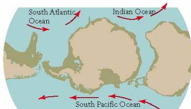
A MIDDLE EOCENE
