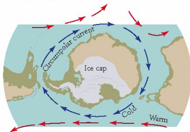
B EARLY OLIGOCENE
